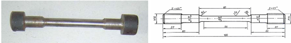
Fig.1 The shape and size of test-bars used in testing
