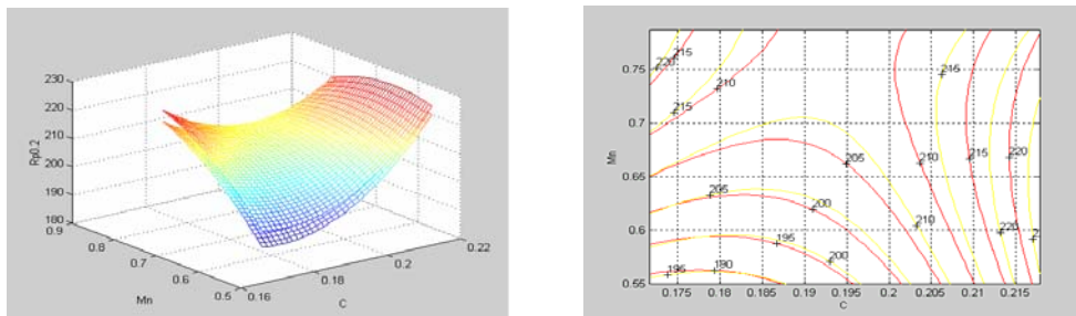
Fig.7 The delimitation of the best field for the technical running limit R_{p0,2/450} , depending on the carbon and manganese content, taking into consideration the medium percentage of silicium
