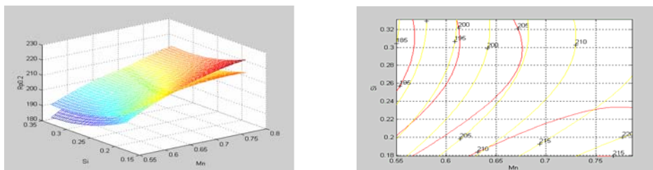
Fig.5 The delimitation of the best field for the technical running limit R_{p0.2/450} , depending on the manganese and silicon content, taking into consideration the medium percentage of carbon
