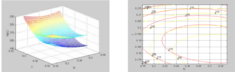
Fig.6 The delimitation of the best field for the technical running limit R_{p0,2/450} , depending on the carbon and silicium content, taking into consideration the medium percentage of manganese
