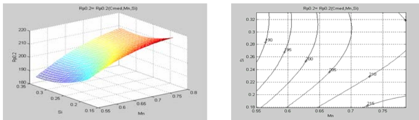
Fig.2 The variation of the technical running limit R_{p0.2/450} , containing manganese and silicon, taking into consideration the medium percentage of carbon
