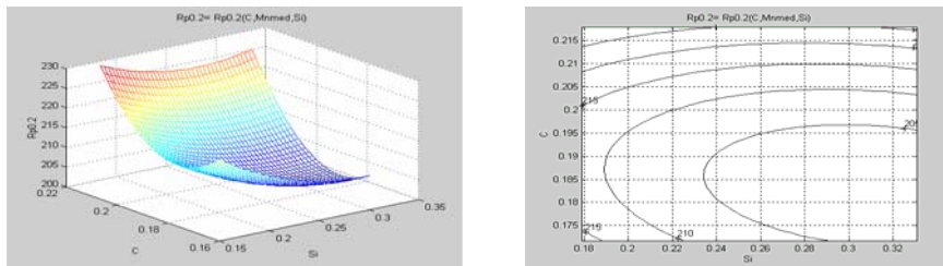
Fig.3 The variation of the technical running limit R_{p0.2/450} , containing carbon and silicon, taking into consideration the medium percentage of manganese
