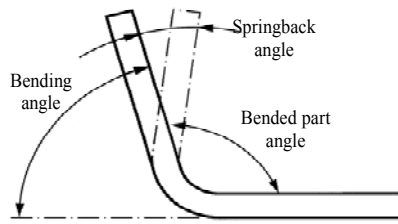
Figure 1. Scheme of the bending process and springback
