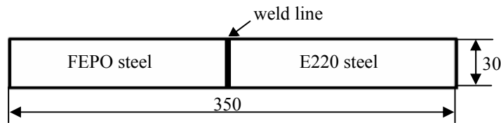
Figure 2. Tailor welded strips with transversal weld line (unit: mm)
