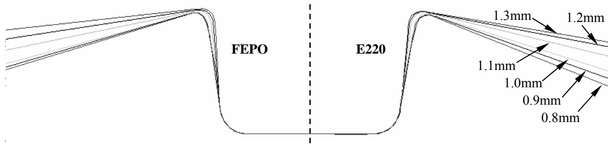
Figure 5. Shape of the TWB deformed by springback phenomenon
