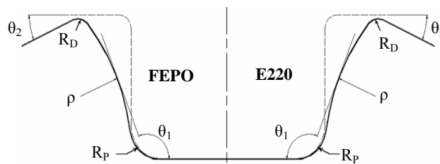
Figure 4. Geometrical springback parameters
