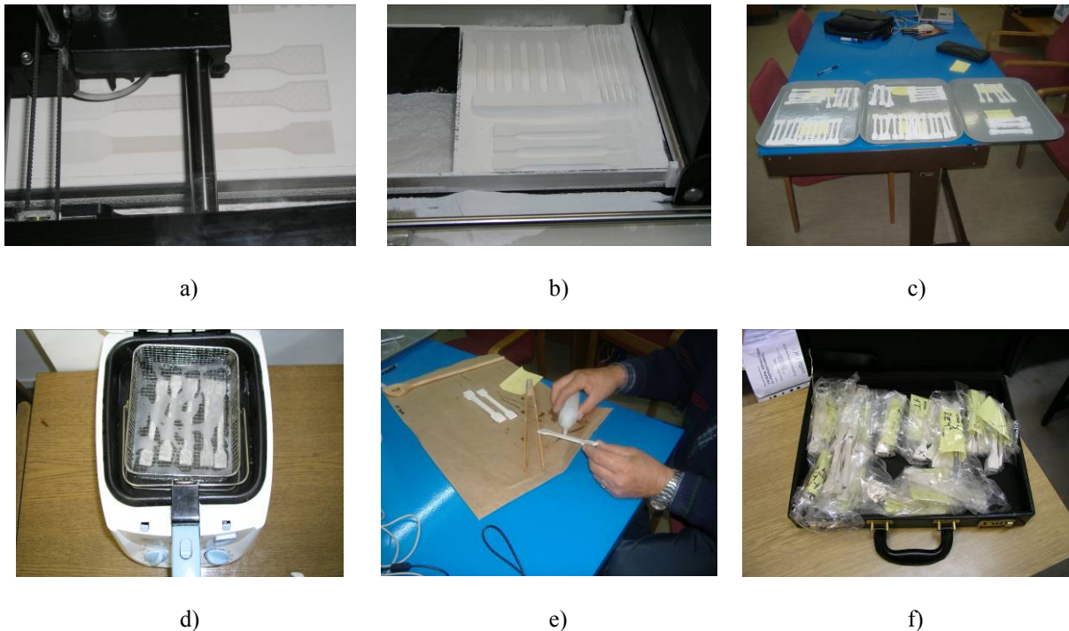
Figure 3.1 Preparation of test pieces: a) printing; b) various model orientation; c) sorted by layer thickness and model orientation; d) wax infiltration; e) cyanoakrylate infiltration; f) sorted and labeled
