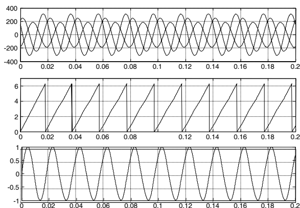
Figure 3 fundamental voltage detection in (V)
