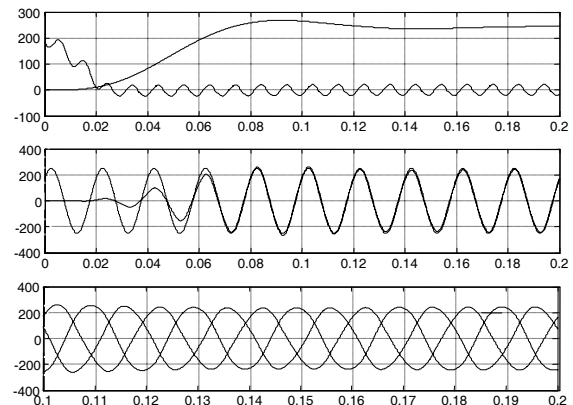
Figure 4 Harmonic current compensation(A)
