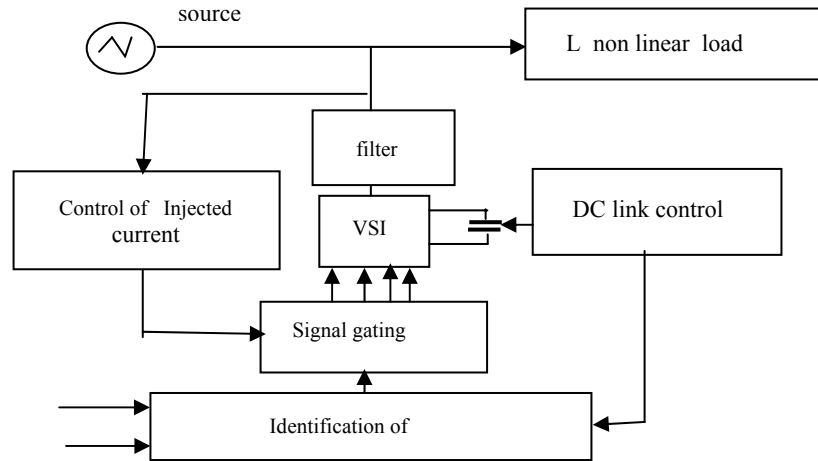
Figure 1. Control schemes of shunt active power filter
