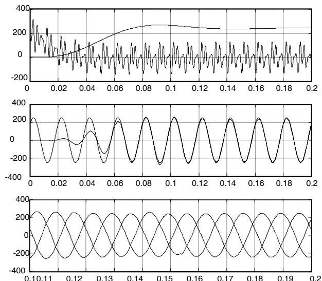
Figure 6 effect of the PLL on current supply
