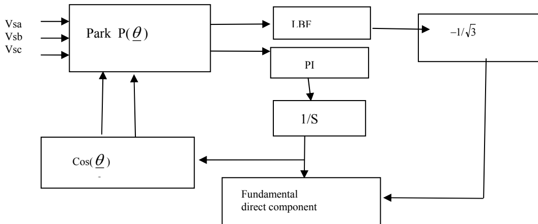
Figure 2. Control scheme of shunt active power
