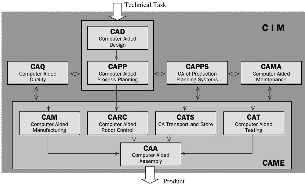
Figure 1. Organization of partially CA systems in CIM complex
