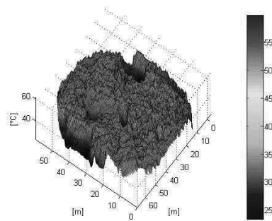
Figure 5. Surface temperatures in 3D [ ^{\circ}\text{C} ]
