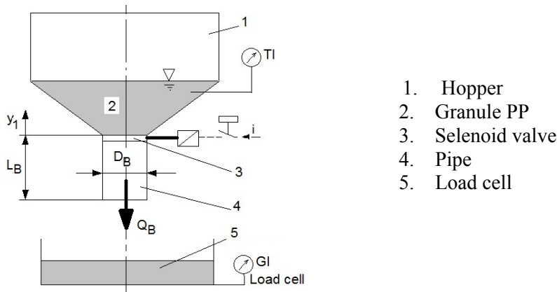
Figure 3. The test equipment of dynamic viscosity
