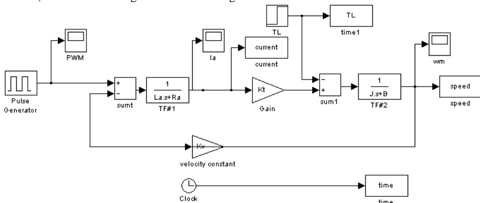
Figure 5. A schematic diagram of a proposed system in MATLAB/SIMULINK
