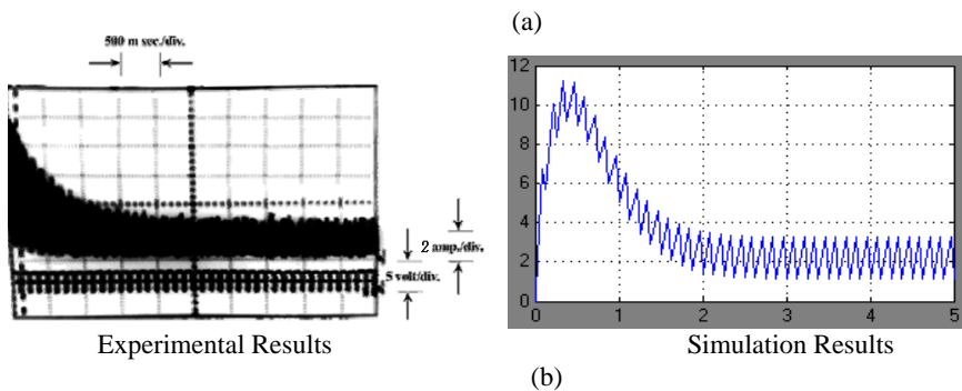
Figure 6. Motor performance of electric vehicle at duty cycle =75% (a) Channel (1): Motor speed (rad./sec.) and Channel (2): Pulses fed to Mosfet driver (b) Channel (1): Motor current (Amp) and Channel (2): Pulses fed to Mosfet driver
