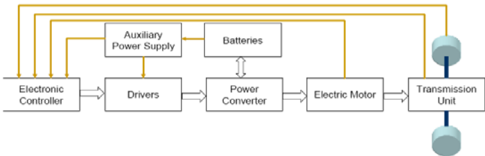
Figure 1. Major Component in an Electric Vehicle
