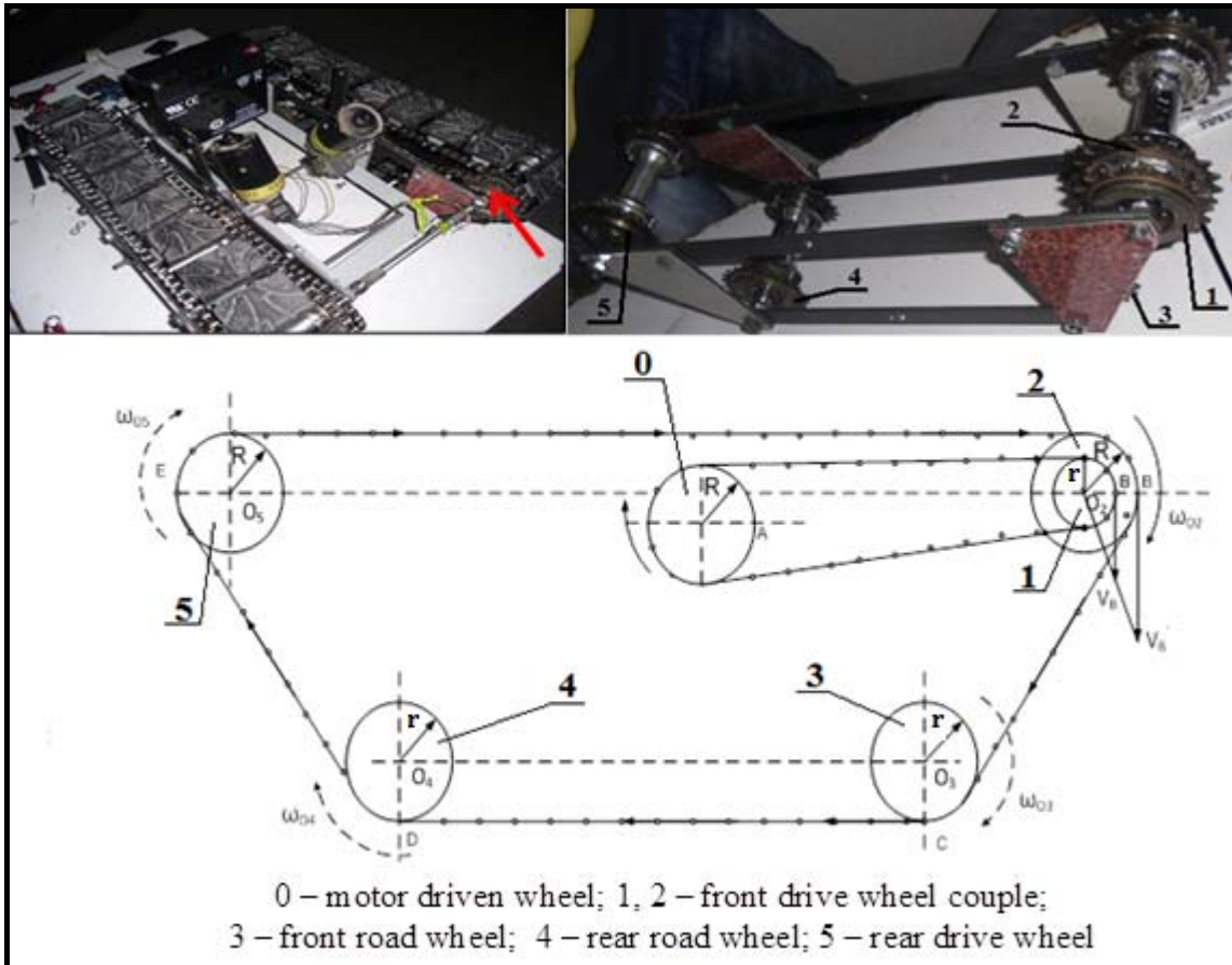
Figure 7. Device and its motion model
