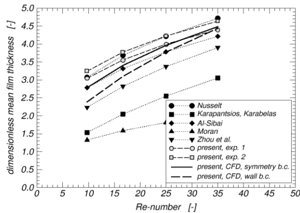
Figure 3. Dimensionless mean film thickness calculated using CFD and compared to experimental results from literature.
