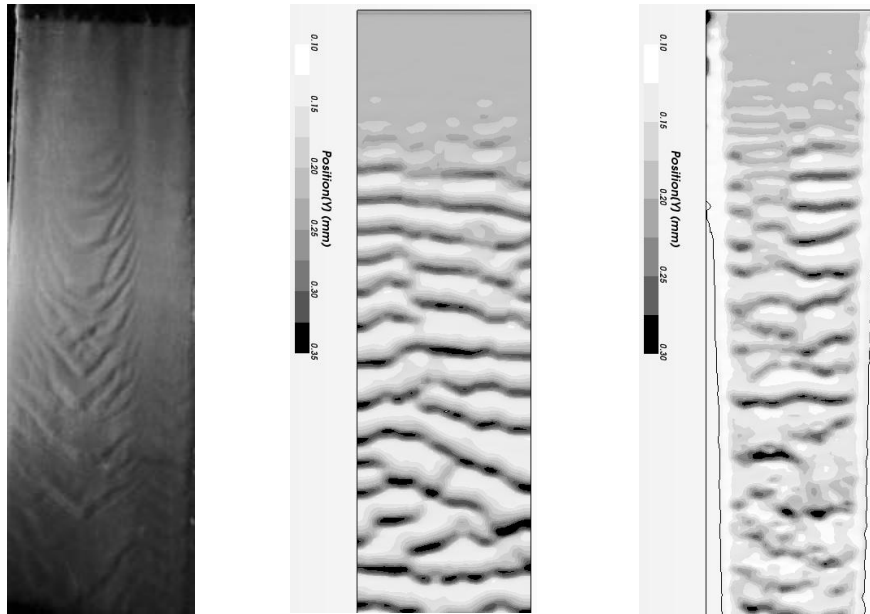
Figure 2. Shape of the free-surface of the liquid film, captured by a camera (left) and obtained from the CFD calculations with symmetry-plane boundary condition at the sides (middle), as well as with wall boundary condition at the sides (right).
