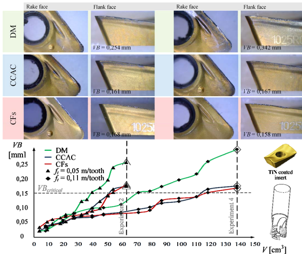
Figure 4. Tool wear progression with volume of the removed material for different machining environments ( v_c = 150 m/min, a_p = 5 mm, a_e = 1 mm, t_{\text{machining}} = 35 min)
