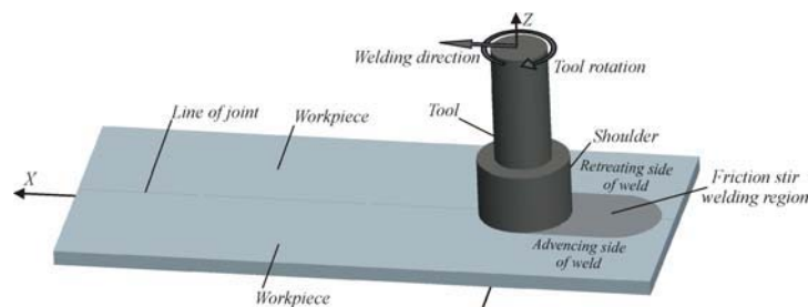
Figure 1. Tool and workpiece [2].
