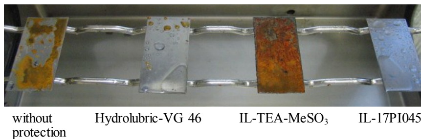
Figure 1. Corrosion testing in a humid chamber
